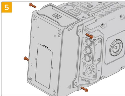
Attach URSA Mini Recorder to the mounting bracket using 2 x T10 torx screws on the left and right side of the brackets.
