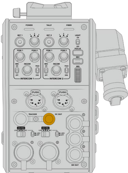
The DC out connector lets you power additional accessories, such as a monitor or external recording equipment
