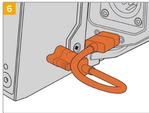
Connect the Mini Recorder's USB-C cable to the USB-C port on the rear of your camera. Tighten the locking connectors with your fingers, or use a 2mm hex key driver. To use with URSA Mini Pro 4.6K G2, use a longer USB-C cable and connect it to the USB-C port above the CFast slots.
