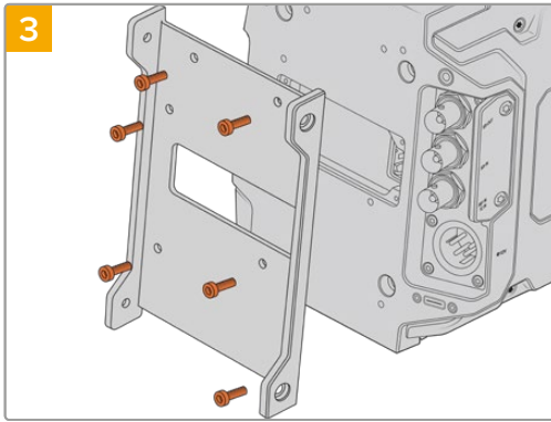
Attach URSA Mini Recorder's mounting bracket using 6 x T10 torx screws.
