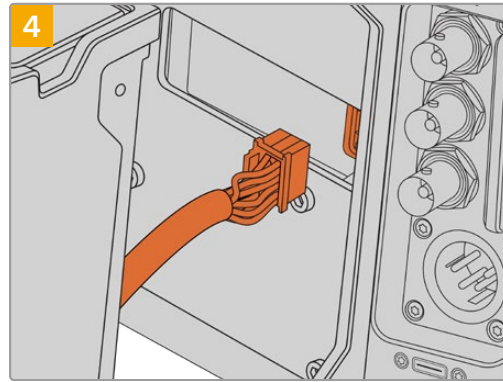
Plug the molex connector on URSA Mini Recorder into the molex socket on your camera's rear panel.
