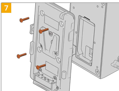
If you want to use a battery plate with URSA Mini Recorder, use a 2mm hex key driver to remove the four M3 screws holding the molex socket cover panel in place. Once the molex socket is uncovered, attach a battery plate using the steps outlined in the section 'mounting batteries' in this manual.
