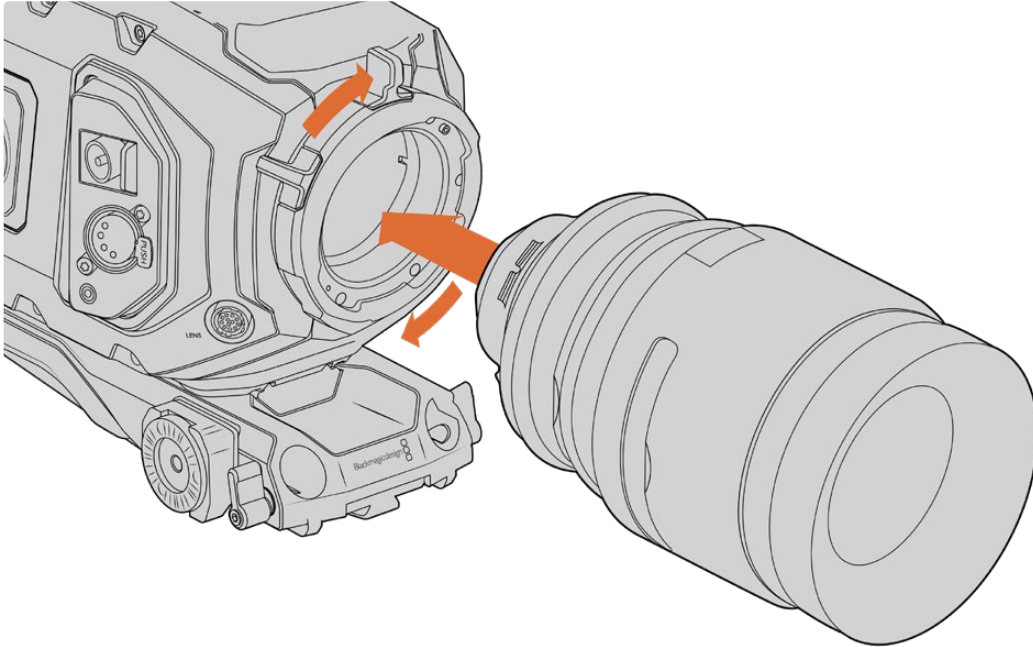
Attaching and removing a PL lens on Blackmagic URSA Mini PL and URSA Mini Pro 12K models
