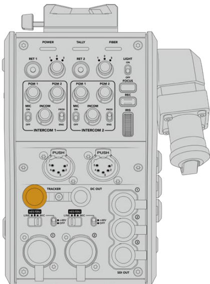
Tracker Interface connector
