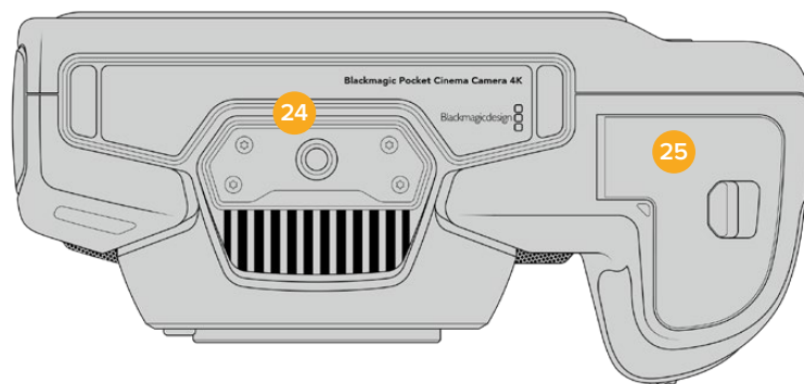
Underside of Blackmagic Pocket Cinema Camera 4K
